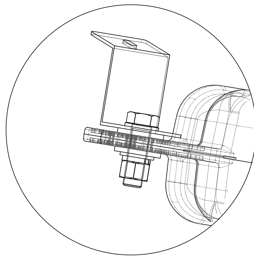
VIEW B
