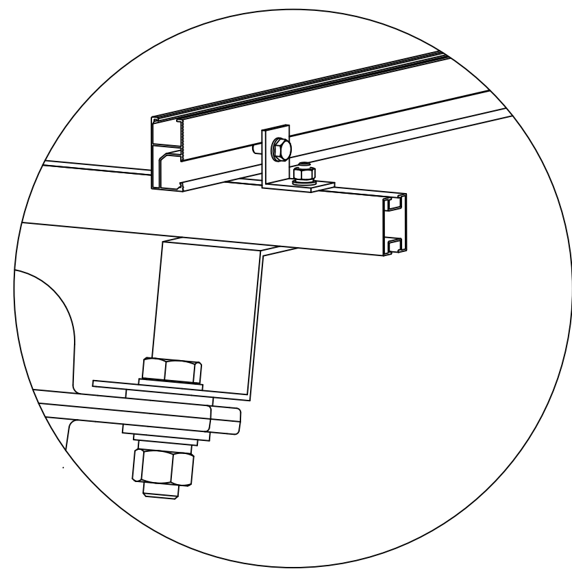
VIEW C
